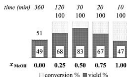
Figure 3. Effect of the MeOH molar fraction
